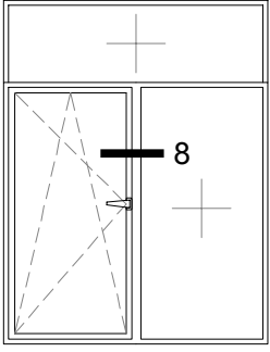
B N L ÇE AÇILIR ORTA KAYITLI DETAY OVERLAPPING INWARD OPENING DETAIL WITH MULLION
