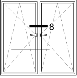
B N L ÇE AÇILIR ORTA KAYITLI DETAY OVERLAPPING INWARD OPENING DETAIL WITH MULLION
