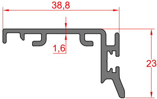
10556 Kenet Profili Interlock Profile Weight : 0,412 kg/mt
