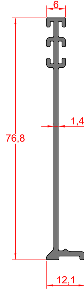
10553 Dikme Profili Mullion Profile Weight : 0,421 kg/mt
