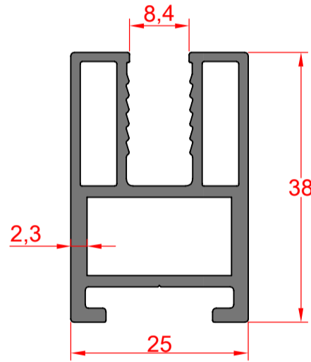
10555 Kanat Profili Sash Profile Weight : 0,761 kg/mt
