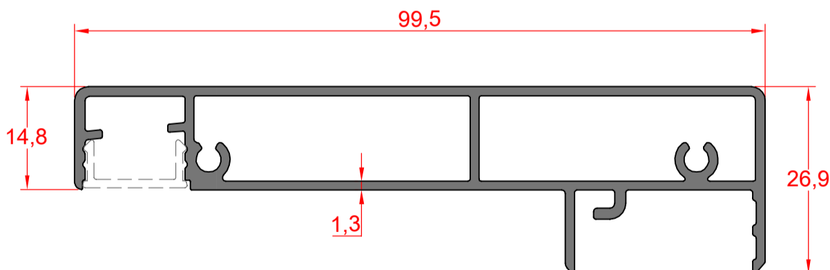
10559 Yatay Profili Transom Profile Weight : 1,045 kg/mt
