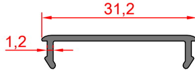
8063 Kanal Kapak Profili Cover Profile Weight : 0,173 kg/mt
