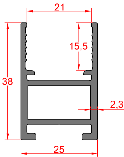
10554 Kanat Profili Sash Profile Weight : 0,637 kg/mt
