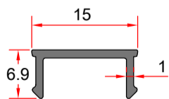
5992 Kapak Profili Cover Profile Weight : 0,080 kg/mt
